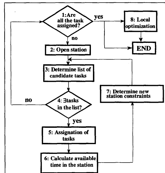
Figure 1: Flow chart for greedy and GRASP approaches.
